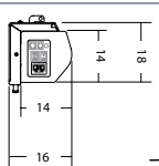
Alimentation Power plug
