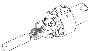
Diagram 11. Connecting to Bridged-Tied Load speakers
