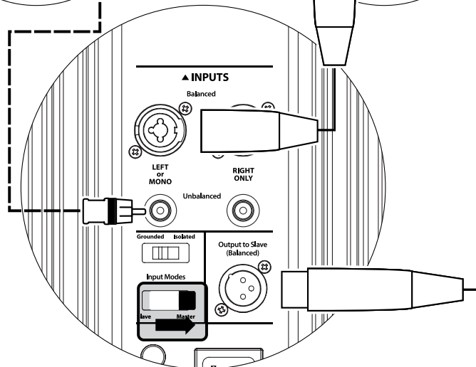
COMANDI POSTERIORI GOTHAM (MASTER)
