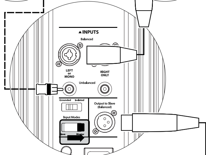
CONTROLES TRASEROS GOTHAM (MAESTRO)
