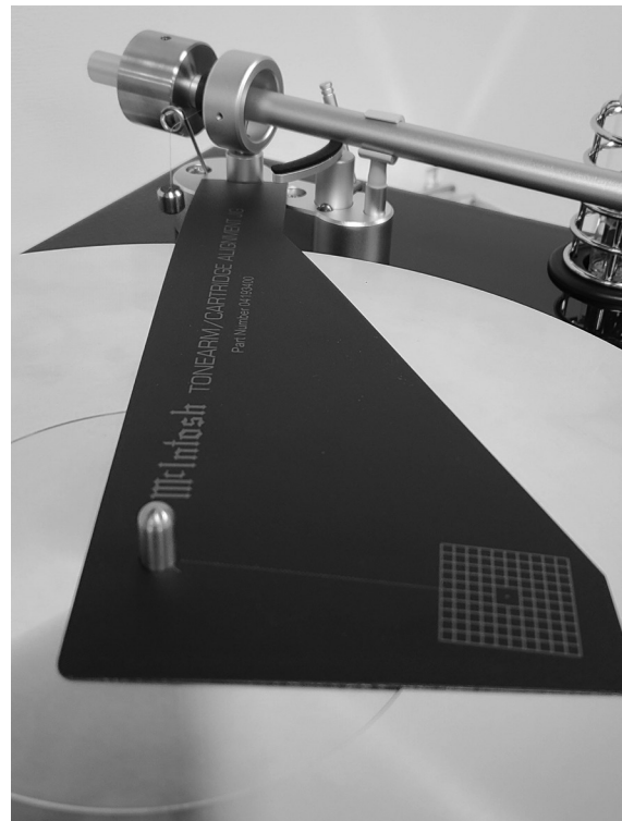
Figure 14– Alignment Jig
