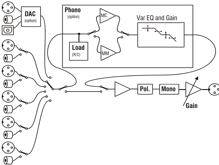
Figure 4: Sketch of the internal signal path.
