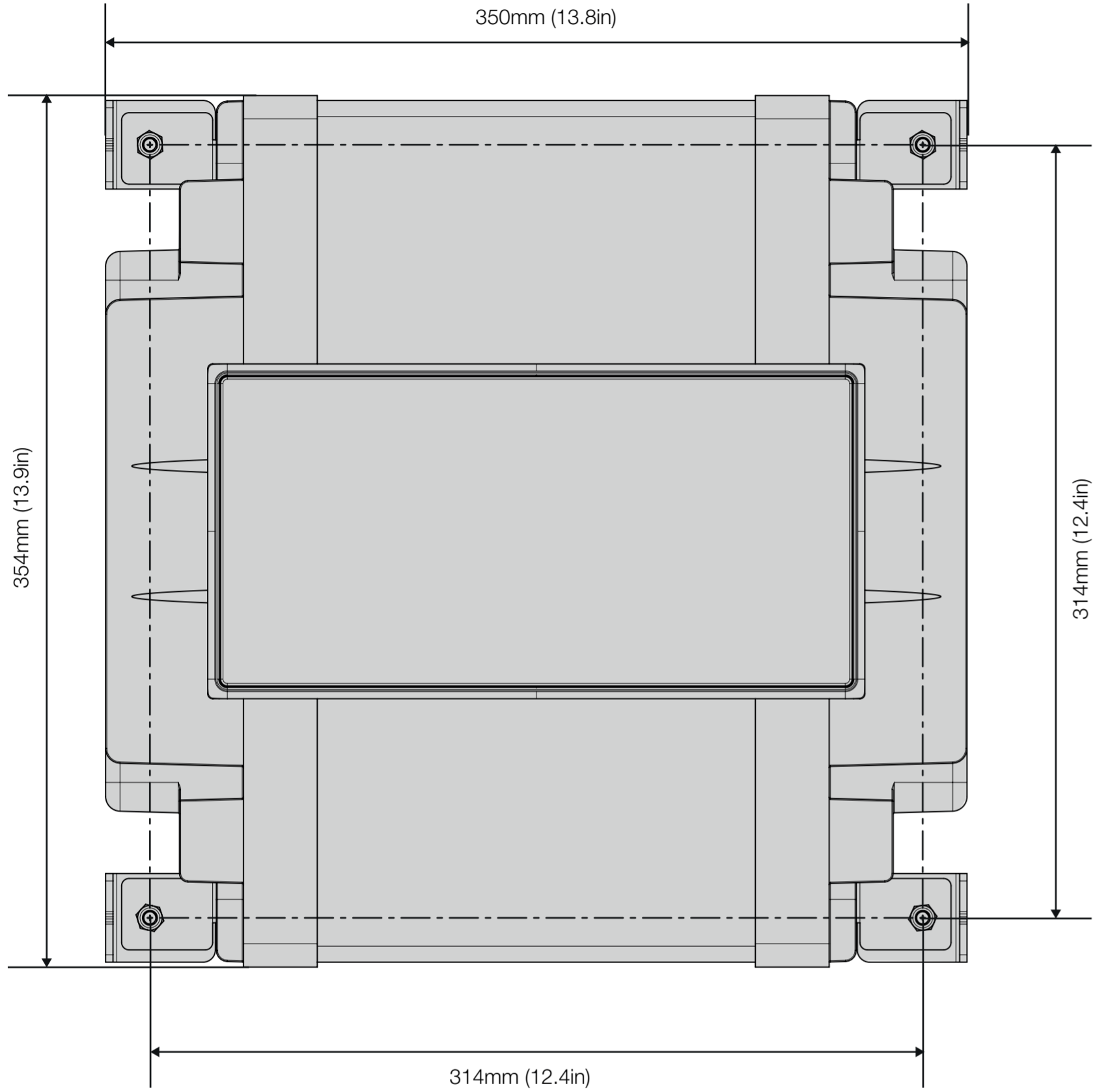
FRONT
