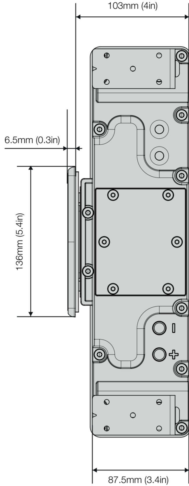
SIDE
